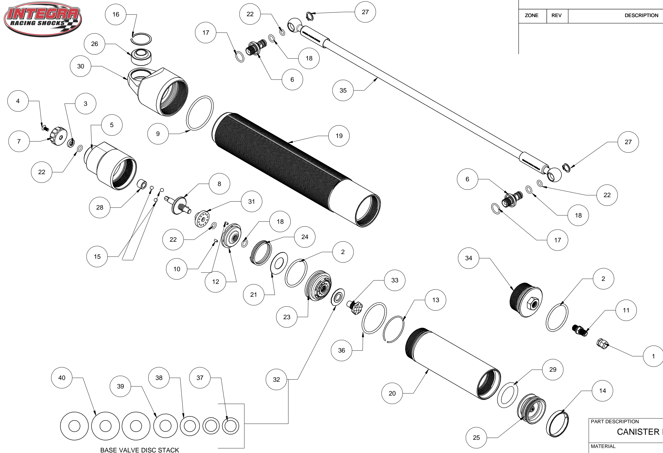
BASE VALVE DISC STACK
